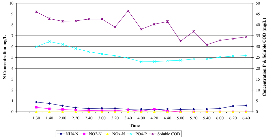
Figure 16. SBR 4A Cycle study 9 th November.
