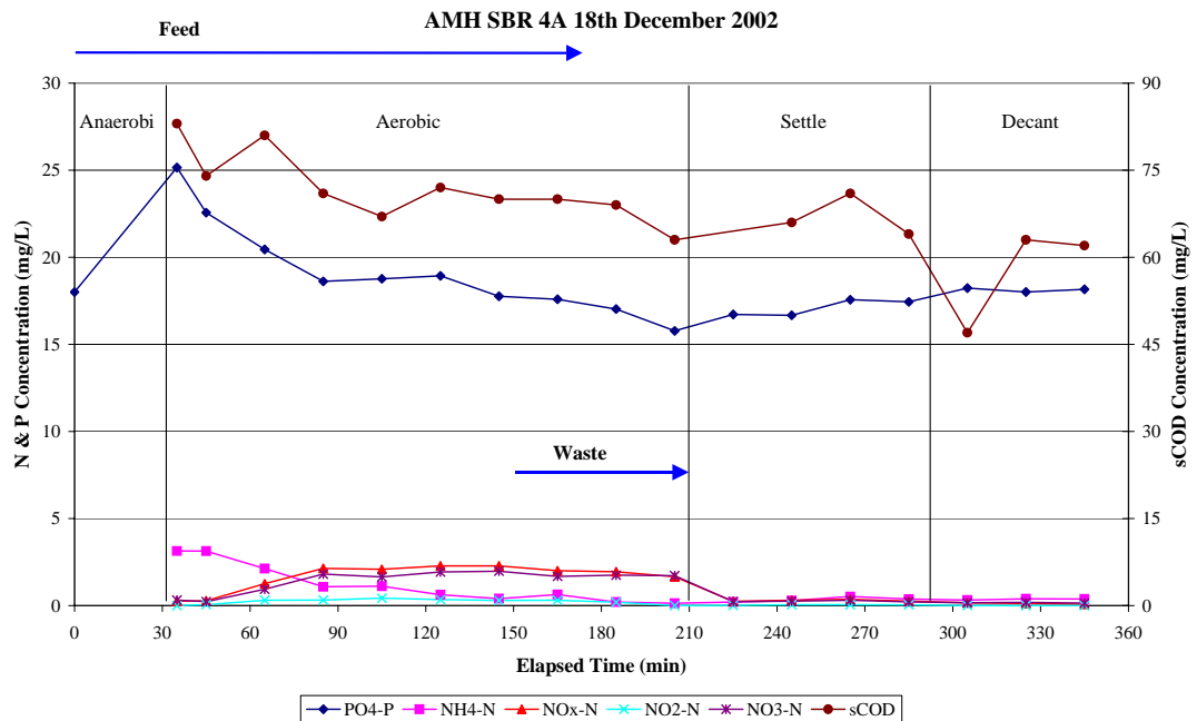
Figure 9. Cycle study on SBR 4A 18 th December 2002
